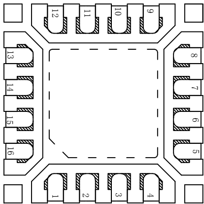
"16L 75X75 QFN (3.0X3.0 PKG)"
